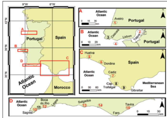
Figure 3.4 Locations where tsunami deposits have been described along the Atlantic Iberia coastline (sandy deposits numbered in red; boulder deposits numbered in black) (adapted from Costa et al., 2012)
