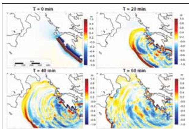
Figure 3.11 Tsunami propagation snapshots for one of the scenarios considered for a tsunami affecting Catania, based on the AD 365 event that occurred off western Crete, Greece and computed by UNIBOL (SCHEMA Report, 2011).
