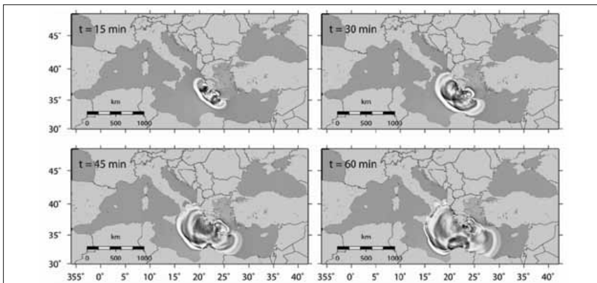
Figure 3.10 Snapshots of the tsunami elevation fields computed for the western Hellenic Arc tsunamigenic scenario (Tinti et al., 2005).
