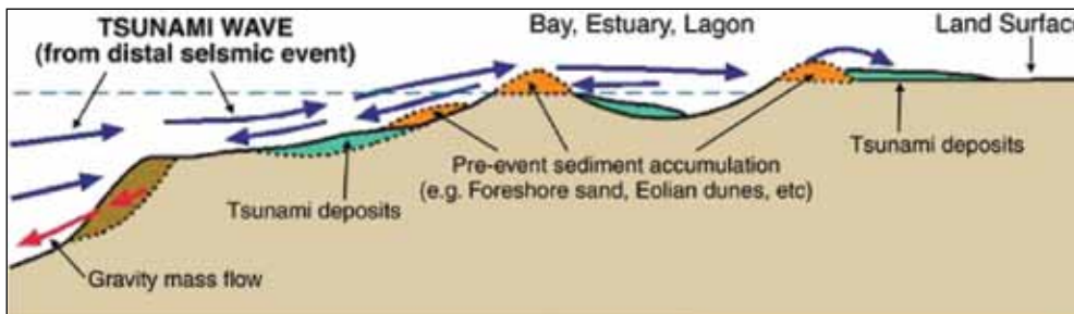
Figure 3.1 Schematic illustration of principal pathways of tsunami sediment transport and deposition (Dawson and Stewart, 2007).
